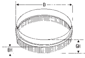
6a-25-6d-50 Topfform/Cup form
