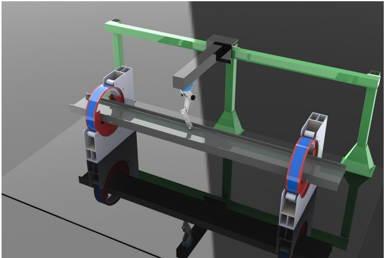
Welding Robotic System for Structural Steel, automatic endplate assembly, automatic attachment assembly
